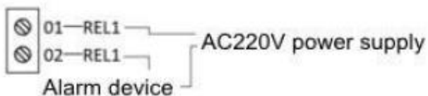
Control alarm wiring
