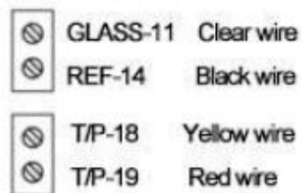
(GRT1010W) Sensor(electrode) wiring
