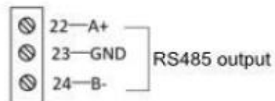
RS485 wiring
