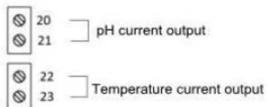
Current output wiring
